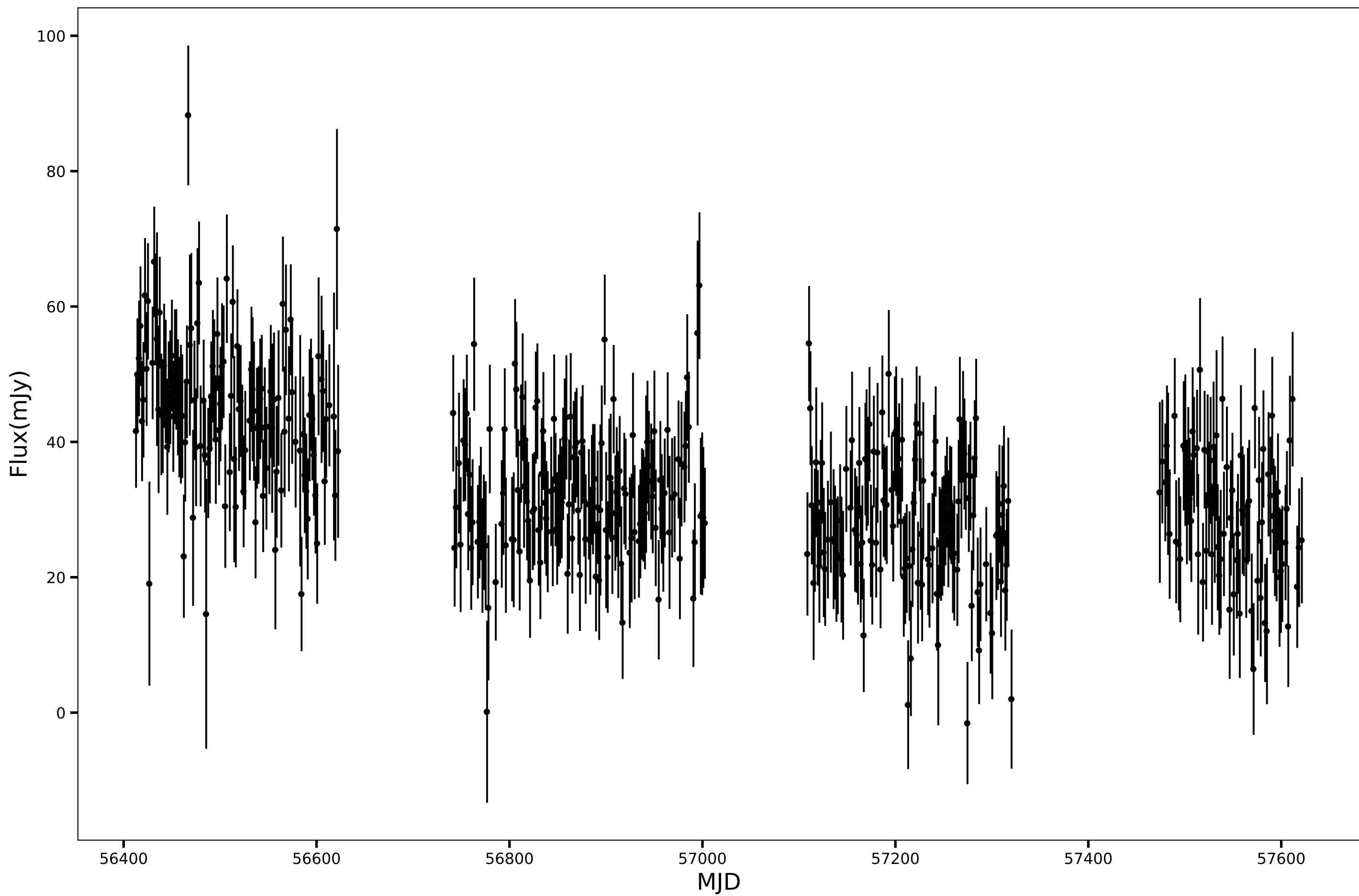
SPT-SJ003735-5307.5, RA=9.3968d, DEC=-53.1261d, mean_flux=33.98 (mJy), 150GHz
