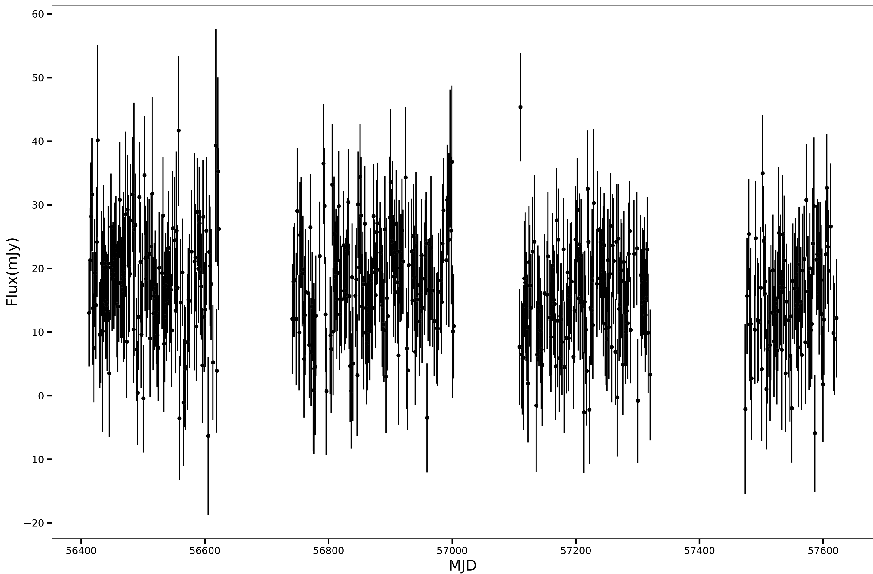
SPT-SJ003725-5917.9, RA=9.3572d, DEC=-59.2997d, mean_flux=16.63 (mJy), 150GHz
