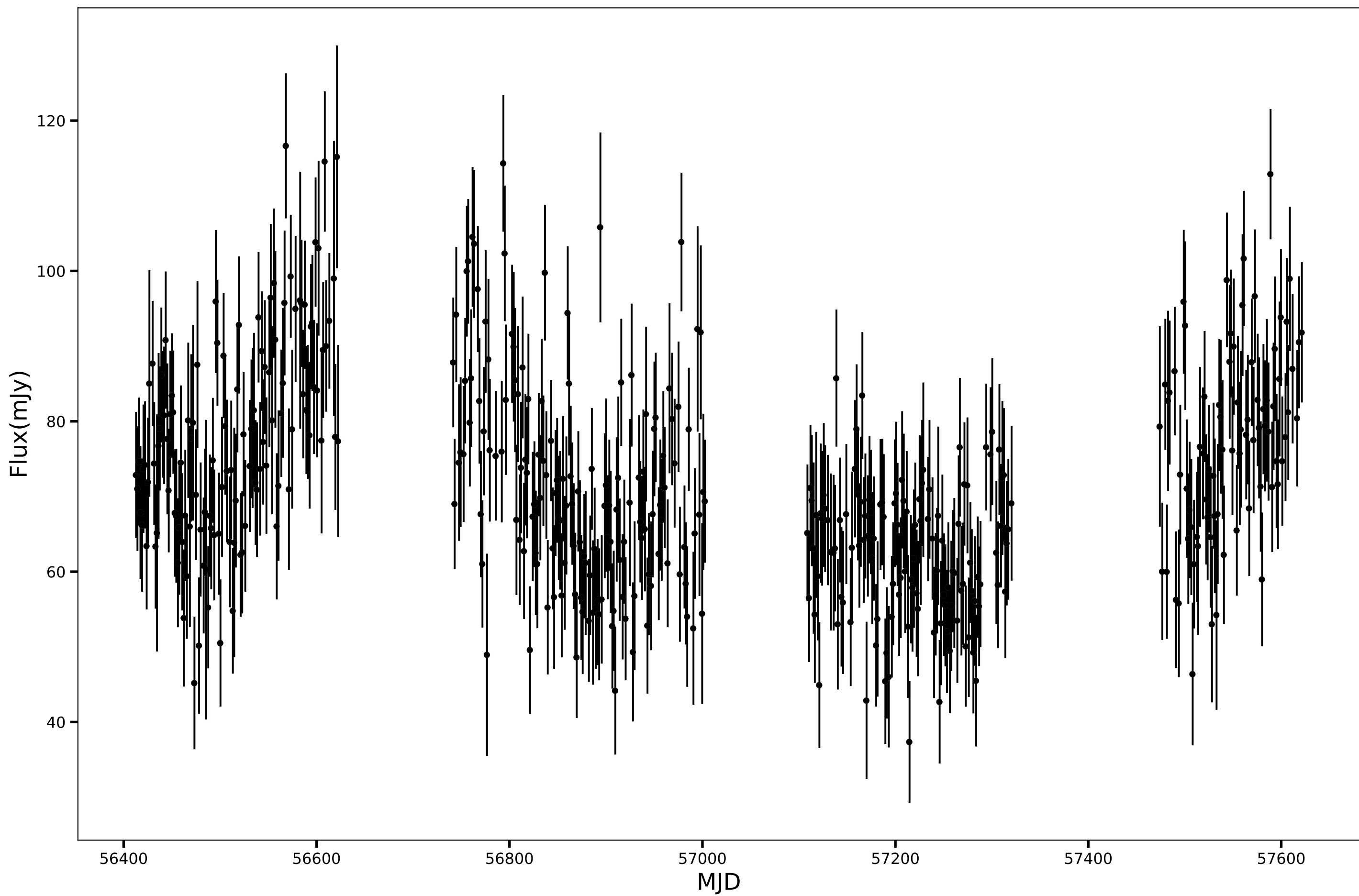
SPT-SJ003133-5143.3, RA=7.8913d, DEC=-51.7229d, mean_flux=71.89 (mJy), 150GHz
