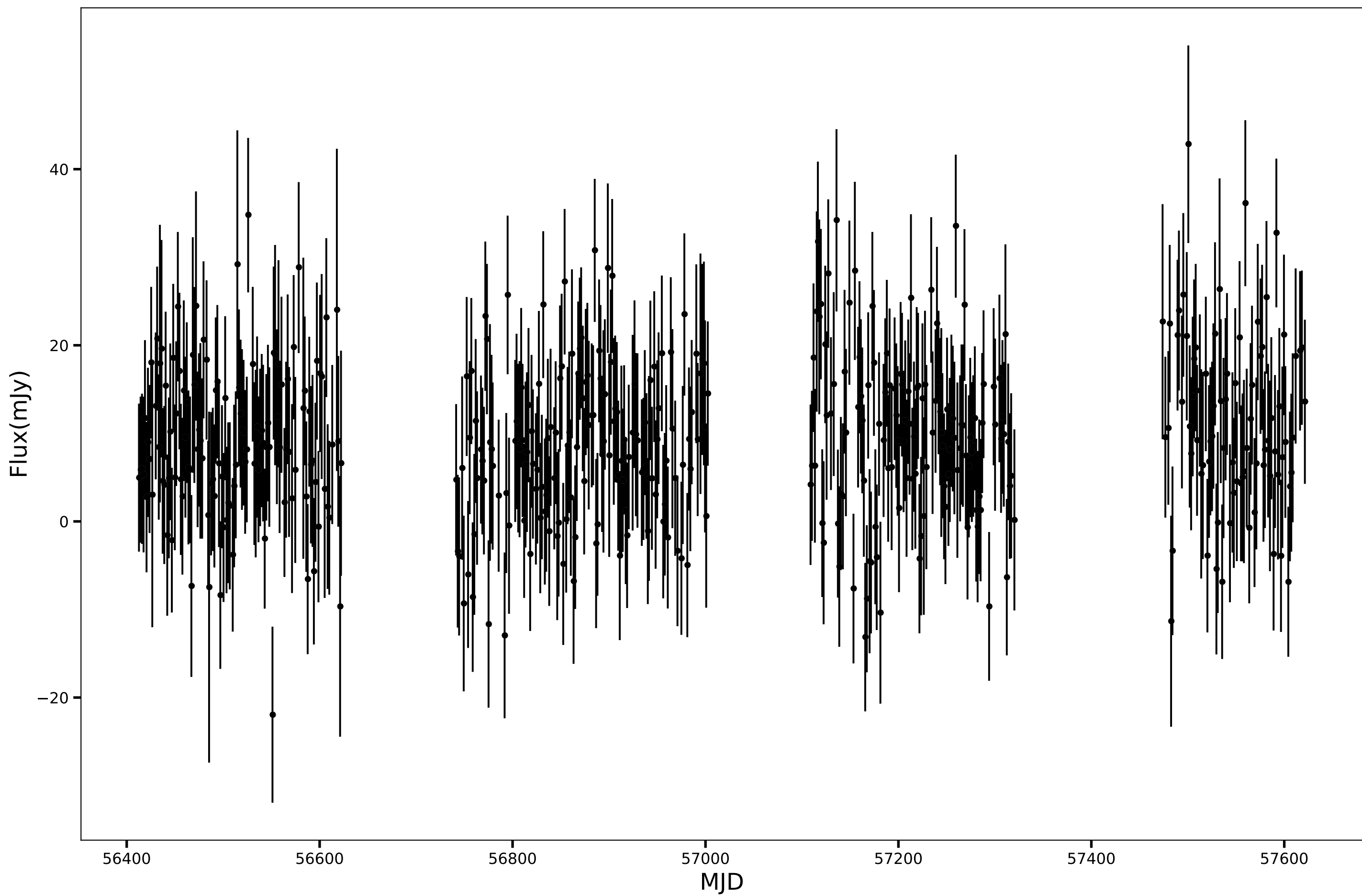
SPT-SJ002736-5409.2, RA=6.9038d, DEC=-54.1545d, mean_flux=9.44 (mJy), 150GHz
