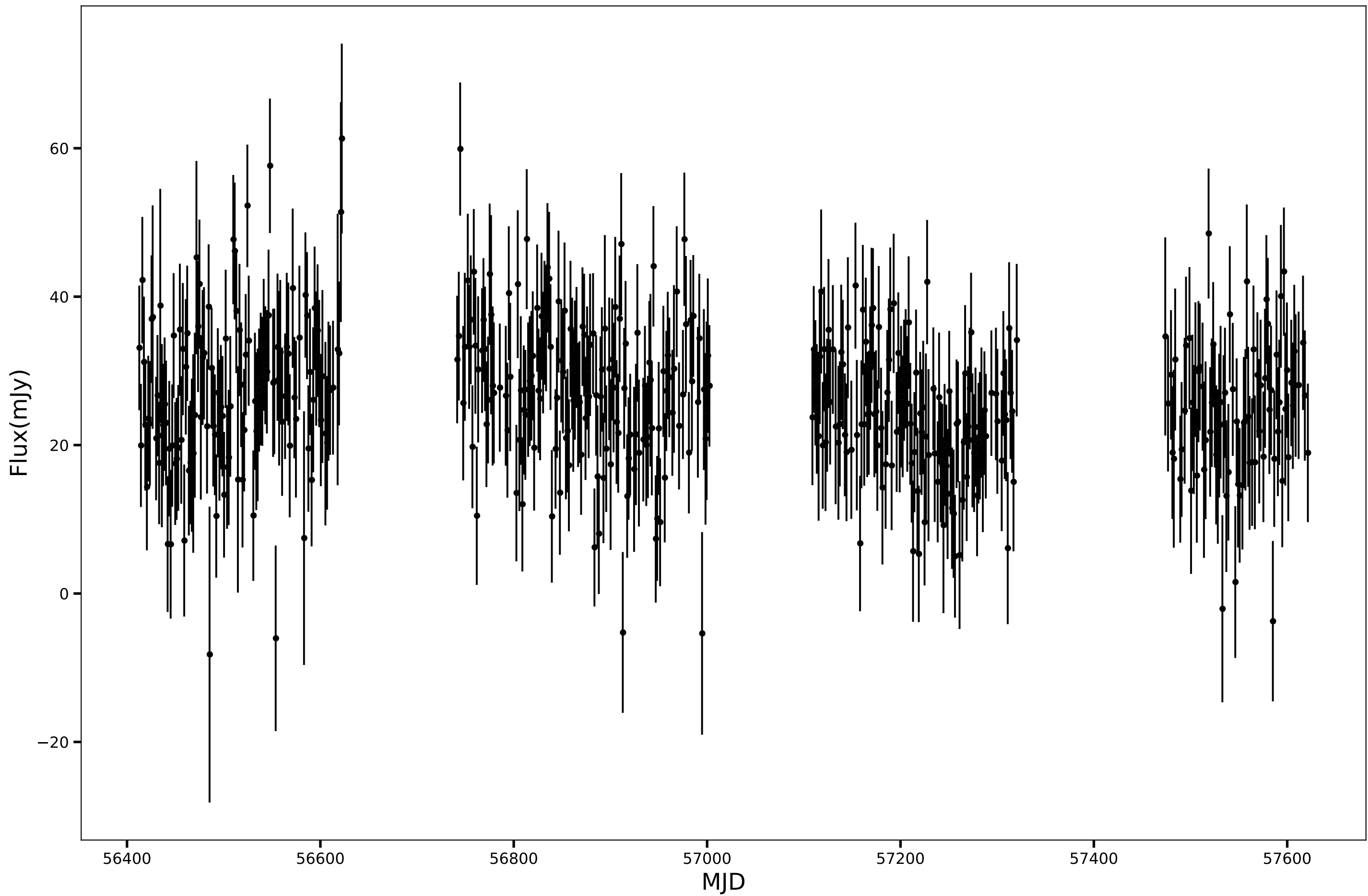
SPT-SJ002510-5427.5, RA=6.2927d, DEC=-54.4599d, mean_flux=25.96 (mJy), 150GHz
