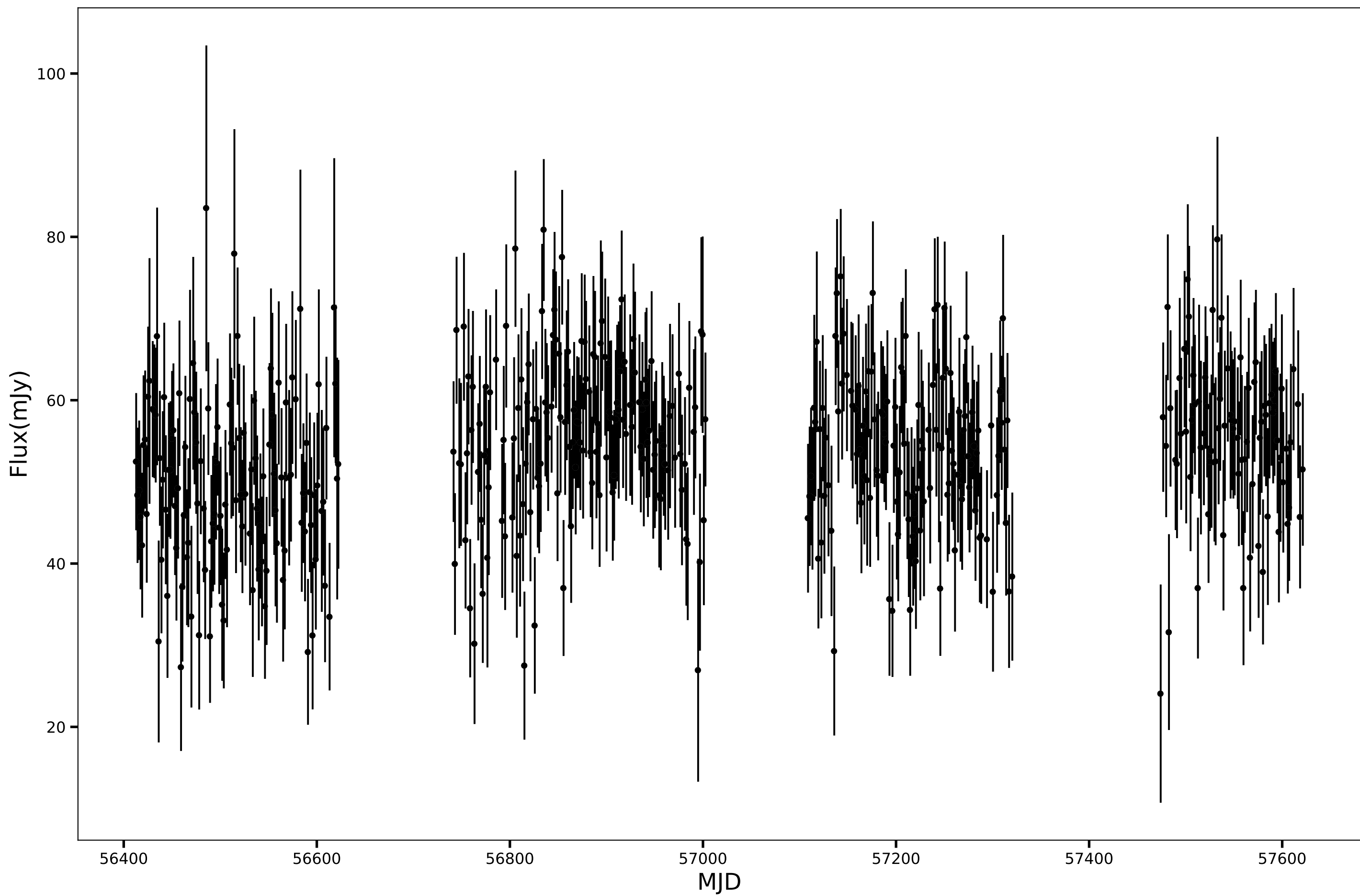
SPT-SJ002302-5650.1, RA=5.7600d, DEC=-56.8355d, mean_flux=53.65 (mJy), 150GHz
