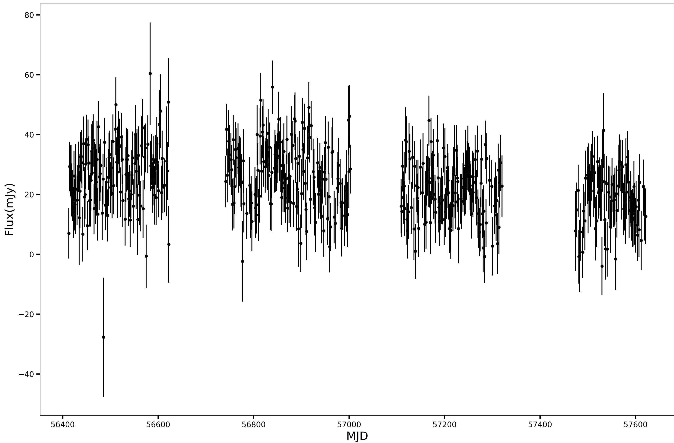
SPT-SJ002233-5153.2, RA=5.6387d, DEC=-51.8871d, mean_flux=23.58 (mJy), 150GHz
