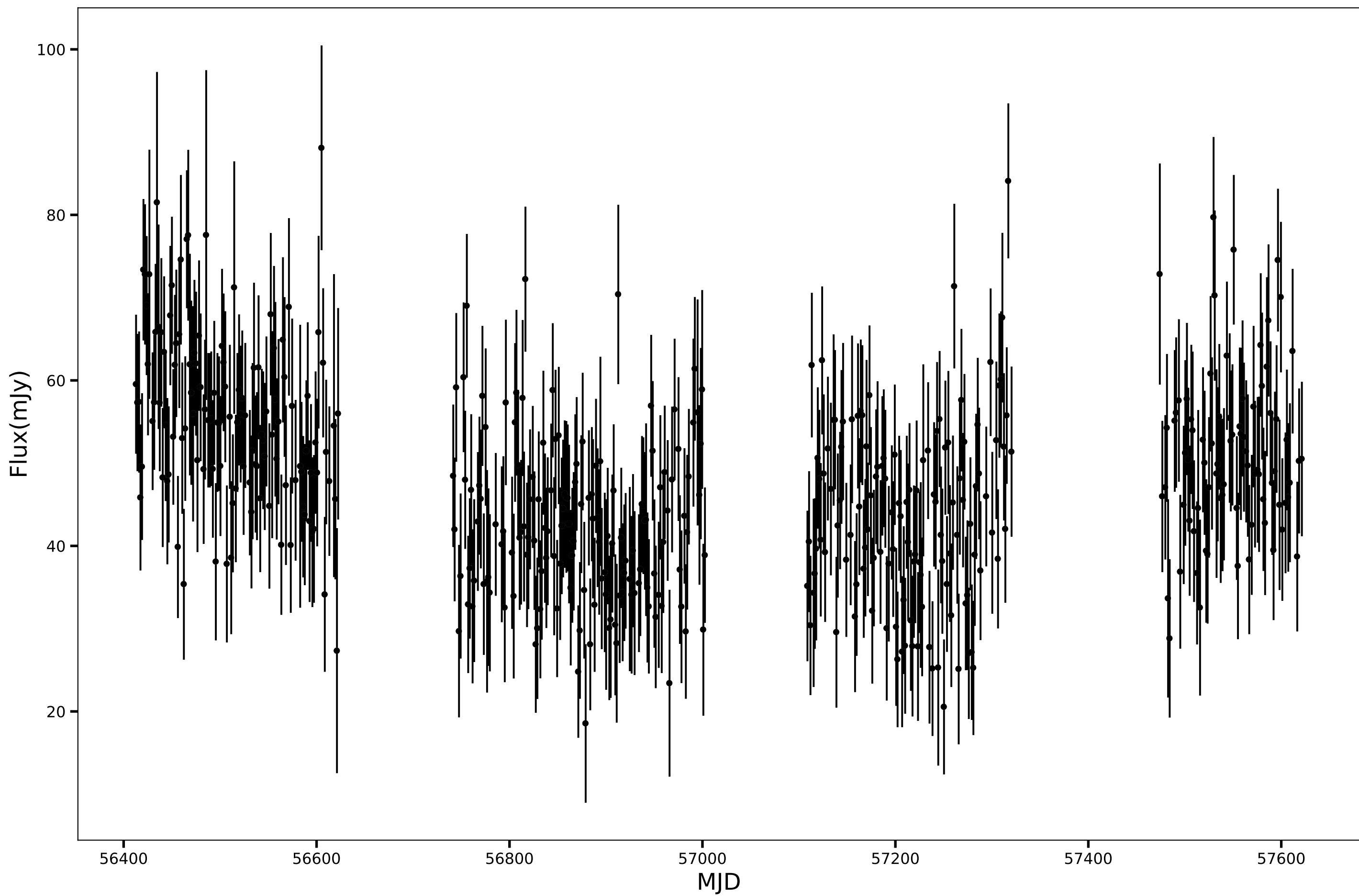
SPT-SJ001848-5115.0, RA=4.7015d, DEC=-51.2506d, mean_flux=47.66 (mJy), 150GHz
