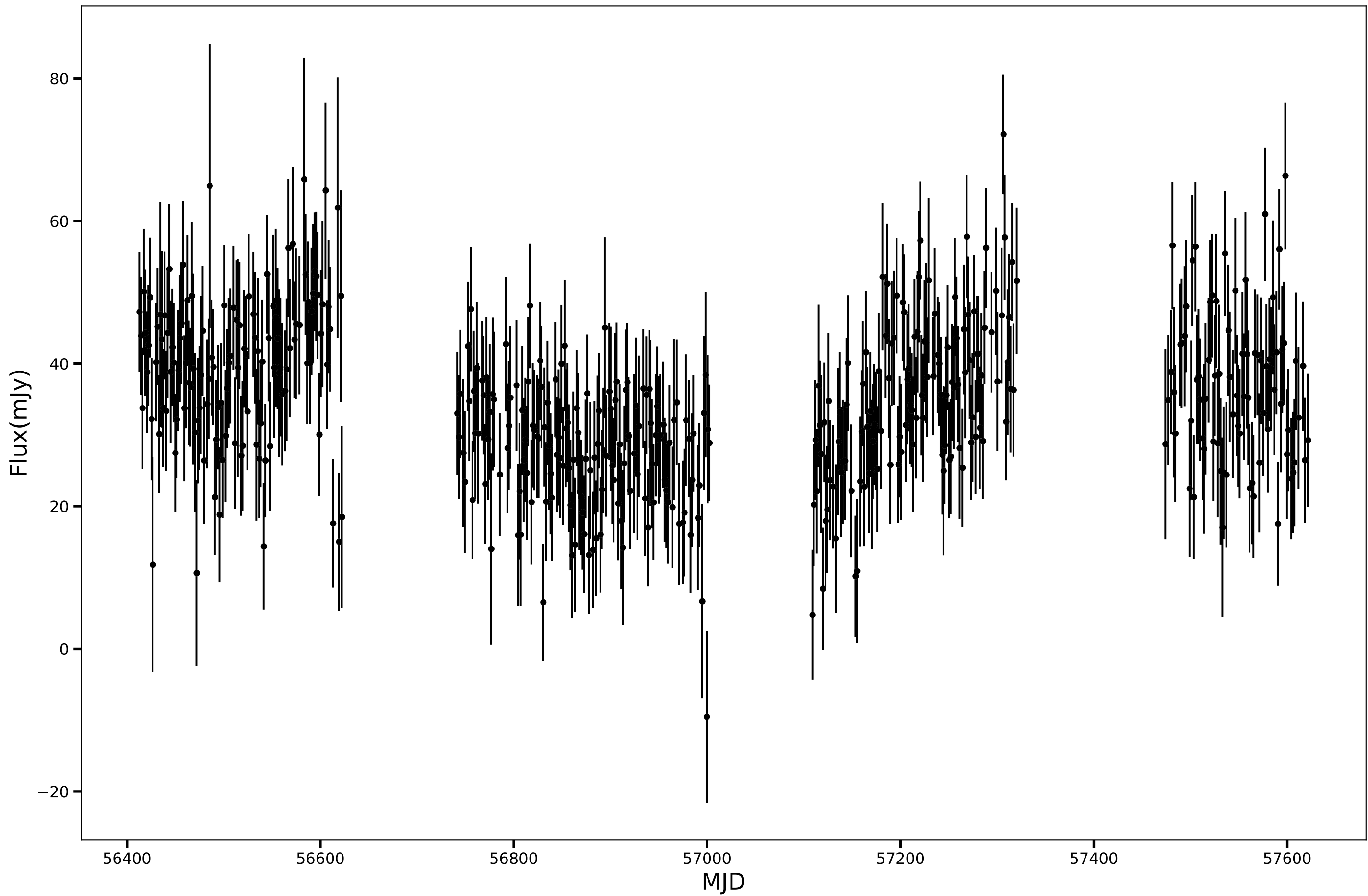
SPT-SJ001426-5638.4, RA=3.6122d, DEC=-56.6404d, mean_flux=34.55 (mJy), 150GHz
