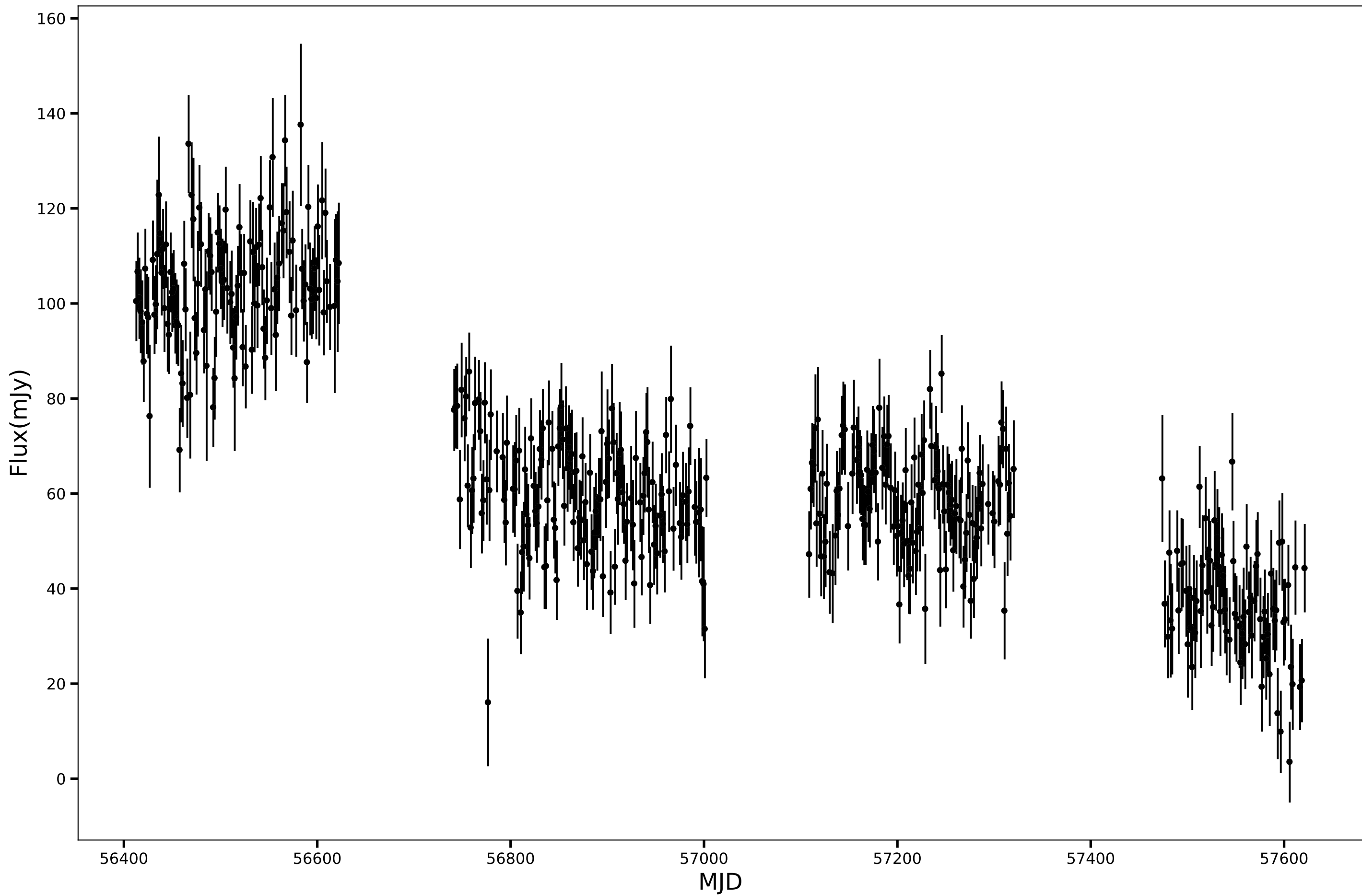
SPT-SJ001324-5005.2, RA=3.3516d, DEC=-50.0877d, mean_flux=67.09 (mJy), 150GHz
