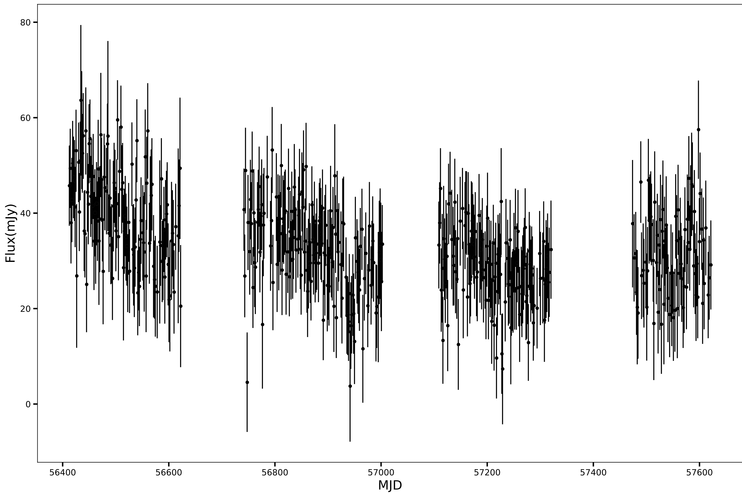
SPT-SJ000936-6357.5, RA=2.4031d, DEC=-63.9591d, mean_flux=33.06 (mJy), 150GHz
