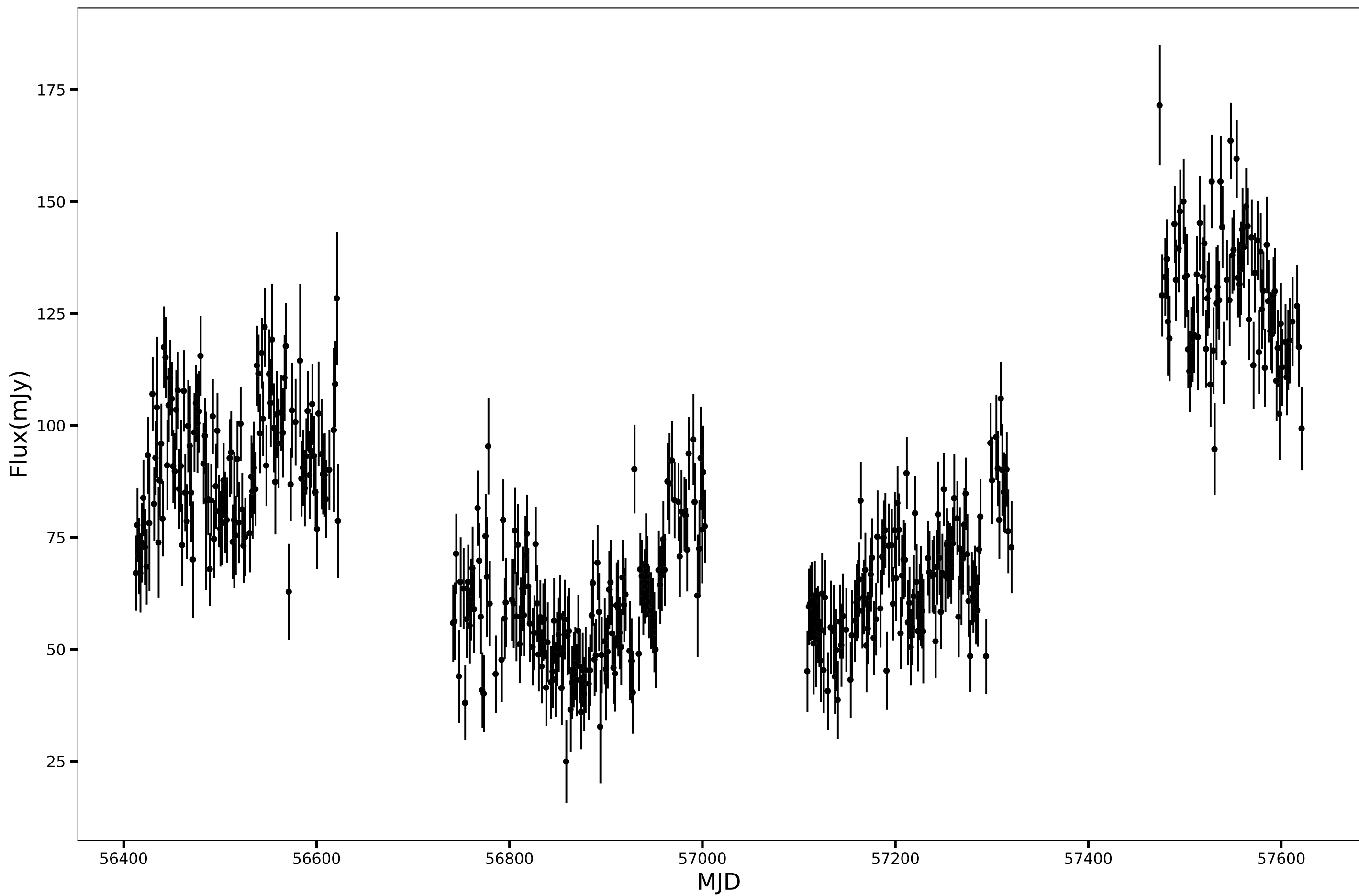
SPT-SJ000800-5243.6, RA=2.0027d, DEC=-52.7277d, mean_flux=81.61 (mJy), 150GHz
