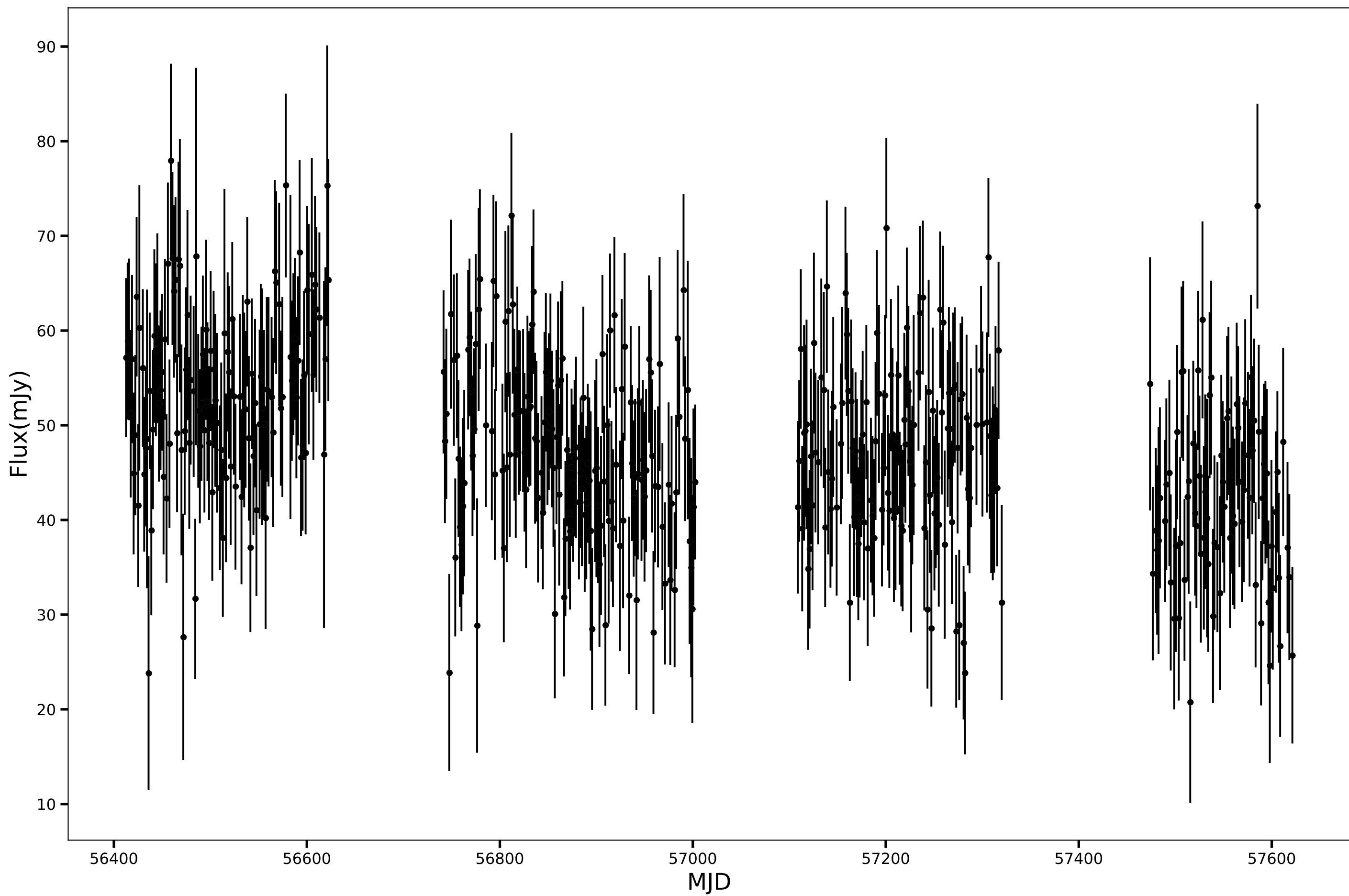
SPT-SJ000719-6113.2, RA=1.8315d, DEC=-61.2210d, mean_flux=47.92 (mJy), 150GHz
