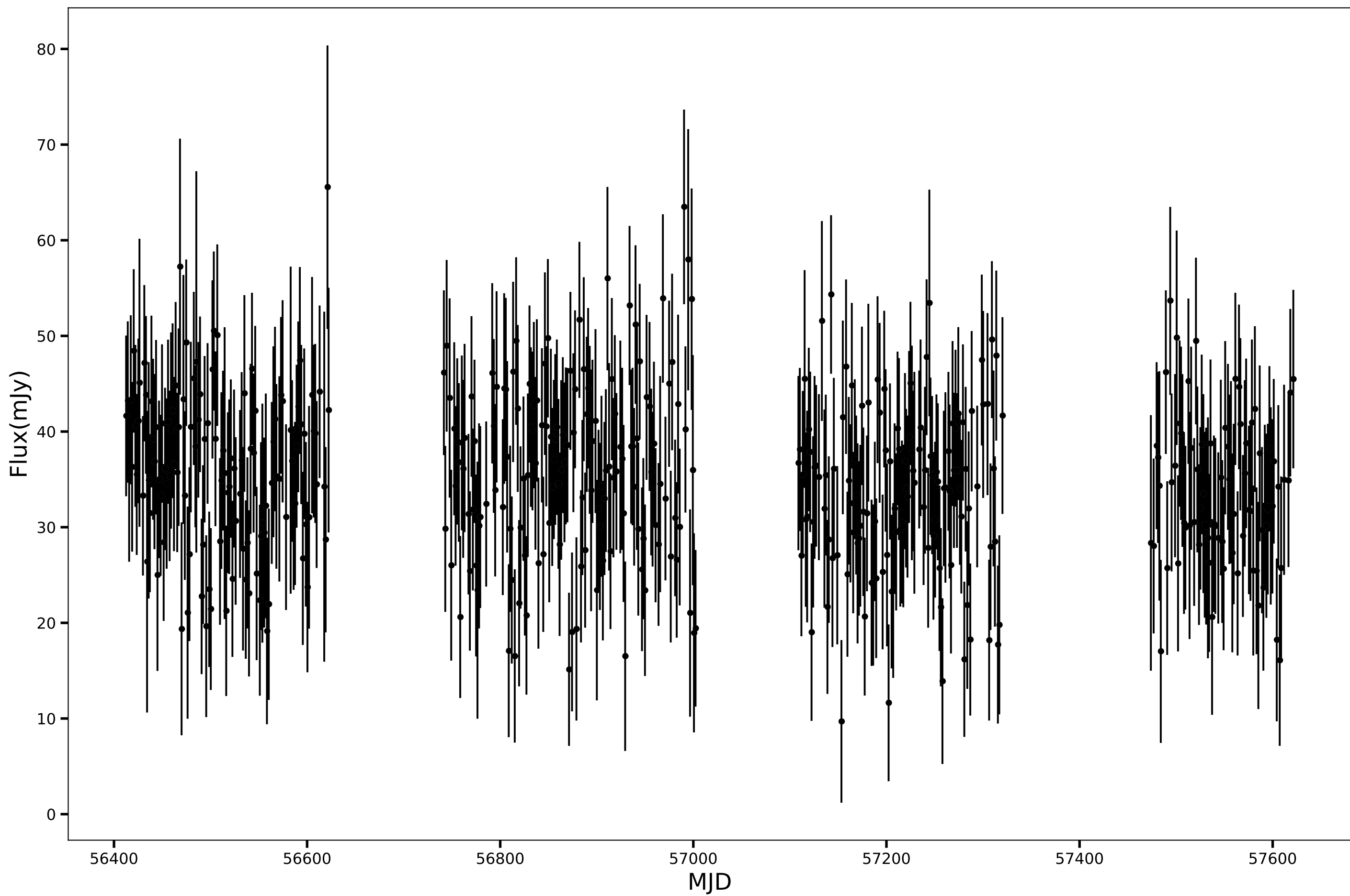
SPT-SJ000558-5628.5, RA=1.4924d, DEC=-56.4755d, mean_flux=35.02 (mJy), 150GHz
