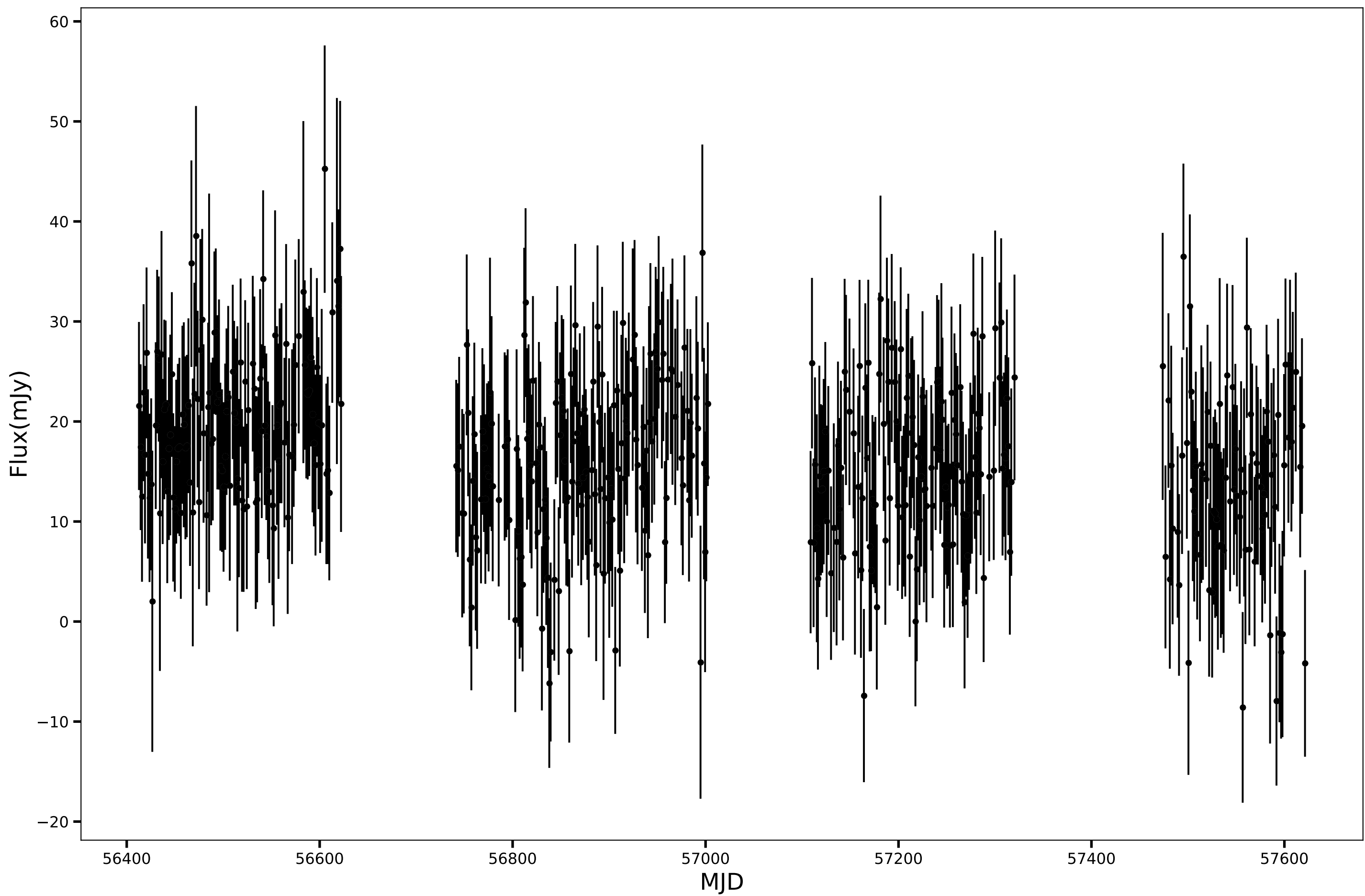
SPT-SJ000312-5905.7, RA=0.8038d, DEC=-59.0958d, mean_flux=16.37 (mJy), 150GHz
