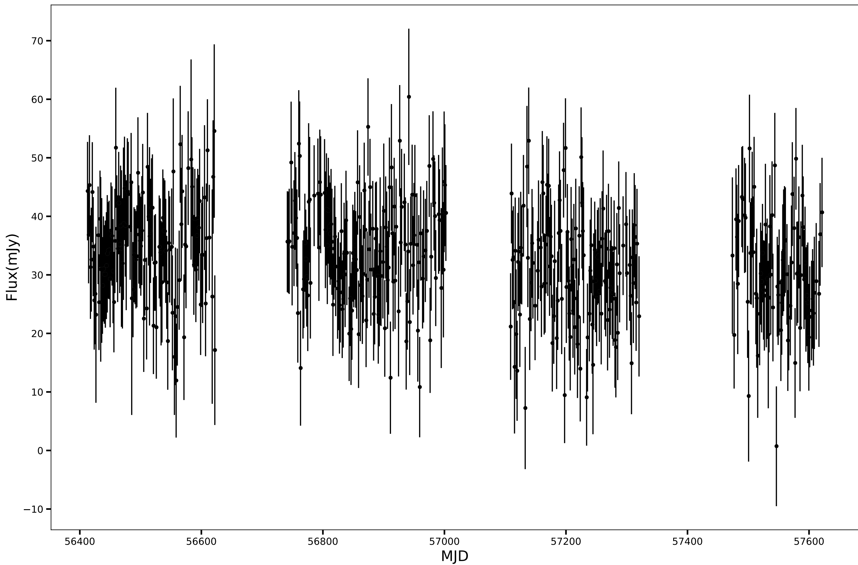
SPT-SJ000310-5444.7, RA=0.7927d, DEC=-54.7461d, mean_flux=32.84 (mJy), 150GHz
