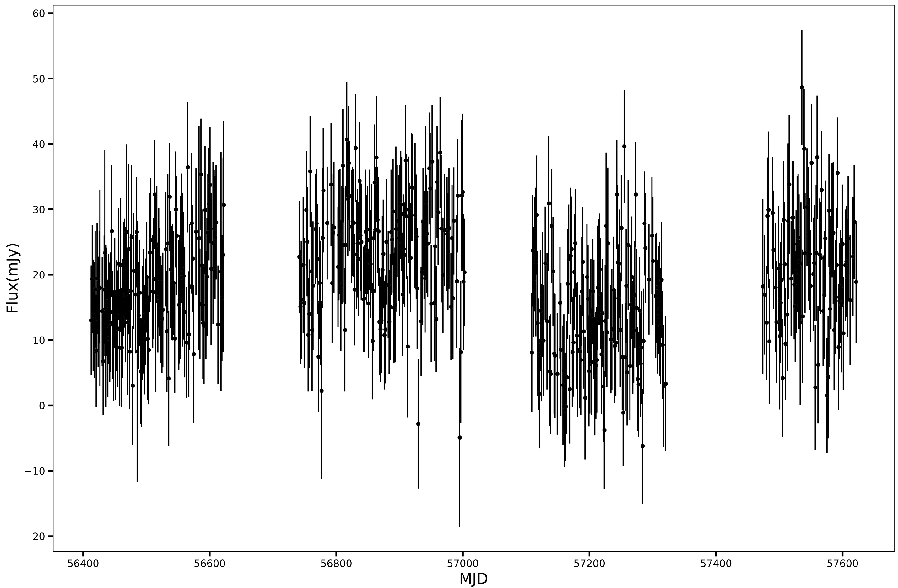
SPT-SJ000303-5529.9, RA=0.7640d, DEC=-55.4997d, mean_flux=19.04 (mJy), 150GHz
